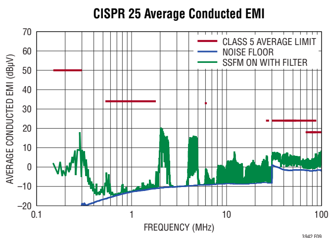
Figure 9. Conducted Average EMI Comparison
