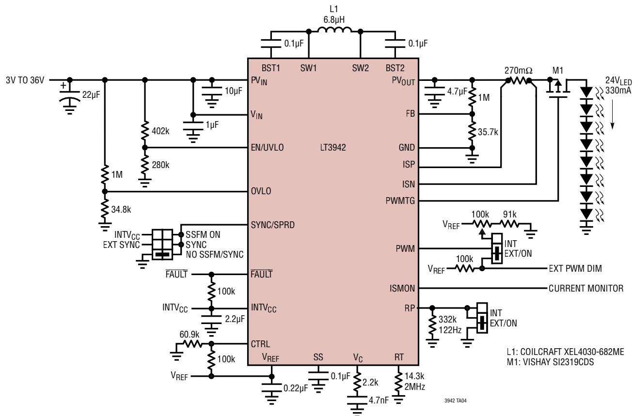
8W (24V, 330mA) 2MHz Buck-Boost LED Driver
