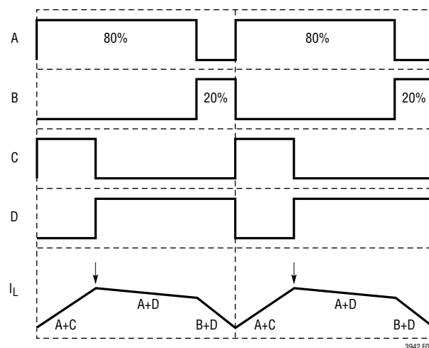
Figure 6. Peak-Boost in Buck-Boost Region ( PV_{IN} \ll PV_{OUT} )
